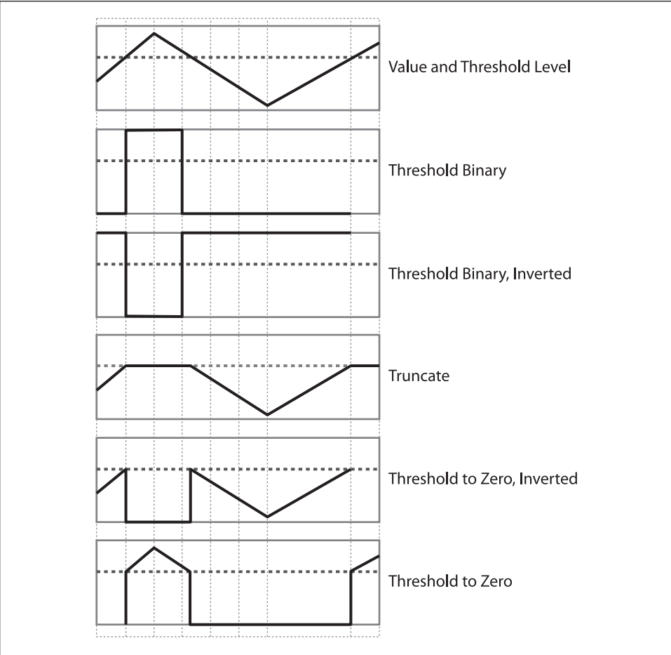
Figure 5-23. Results of varying the threshold type in cvThreshold() . The horizontal line through each chart represents a particular threshold level applied to the top chart and its effect for each of the five types of threshold operations below
