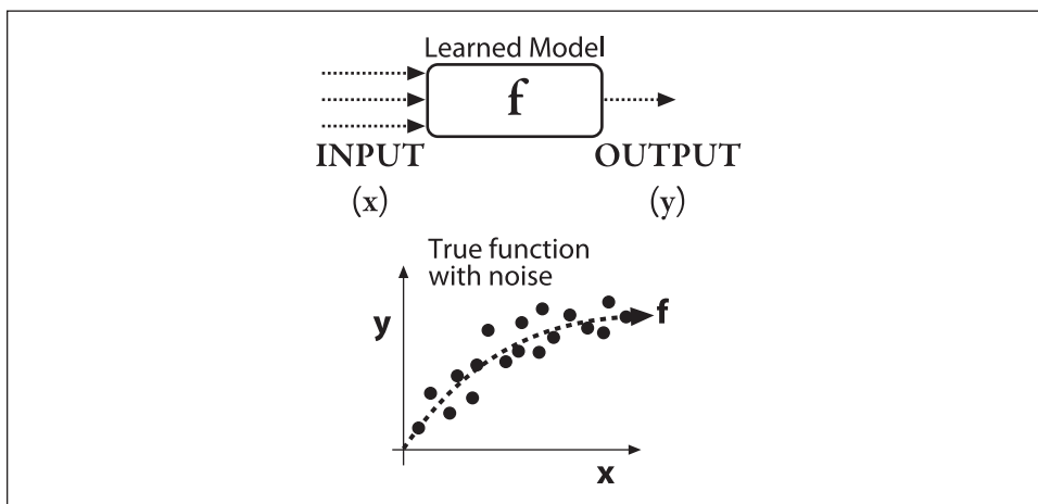
Figure 13-1. Setup for statistical machine learning: we train a classifier to fit a data set; the true model f is almost always corrupted by noise or unknown influences
