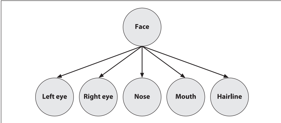
Figure 13-6. A (naïve) Bayesian network, where the lower-level features are caused by the presence of an object (the face)
